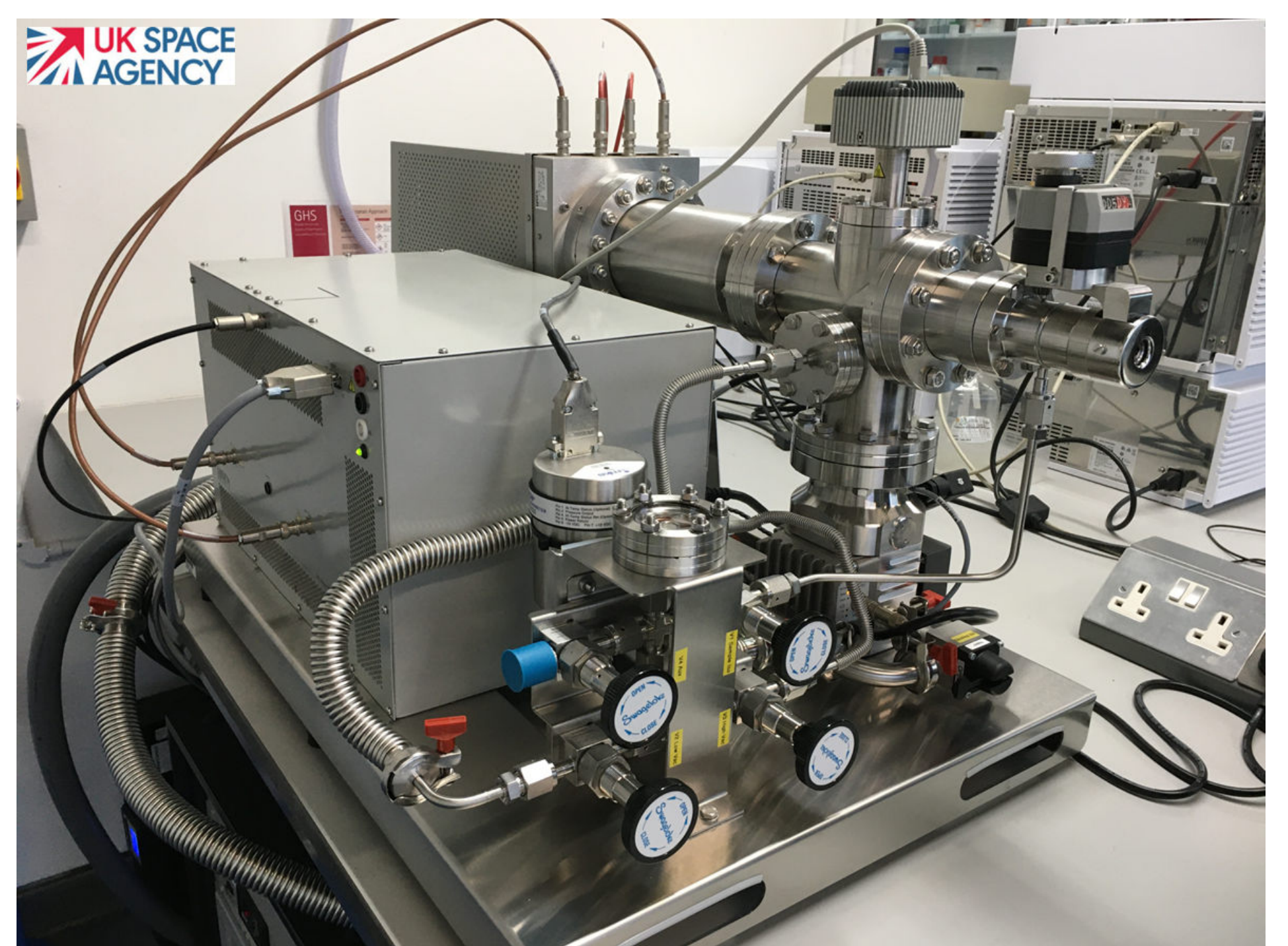
Fig. 2: Vacuum chamber for seed samples with options for analyses of seed volatiles released under low pressure: Mass Spectrometry (MS) and Gas Chromatography Mass Spectrometry (GC-MS). The equipment and associated GENESSIS pre-flight experiments are funded by the UK Space Agency (UKSA).
