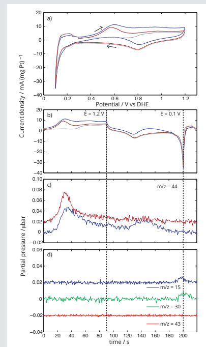
Cyclic Voltammograms recorded in a fuel cell at 80^\circ\text{C} and 90%RH, at a scan rate of 10\text{ mV s}^{-1} and selected m/z signals.
