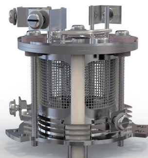
UHV vacuum fired source
