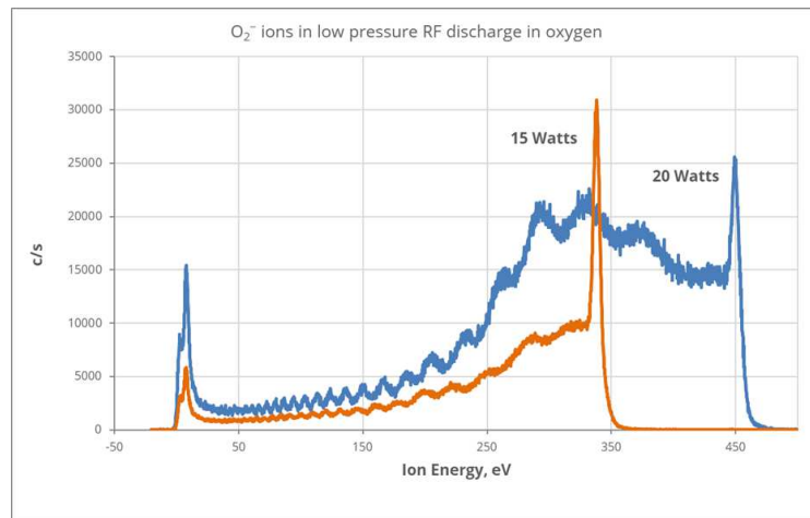
Ion Energy Distribution Scans (IEDs)
