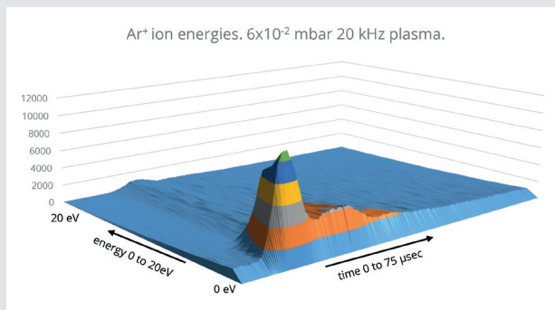
Ion energy distribution of argon ions with respect to time after the onset of a plasma pulse.
