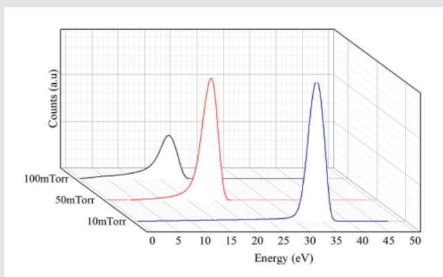
IEDs as a function of pressure in 1000 W Ar.
