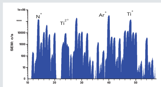
Time averaged mass spectrum from a titanium nitride HiPIMS plasma.
