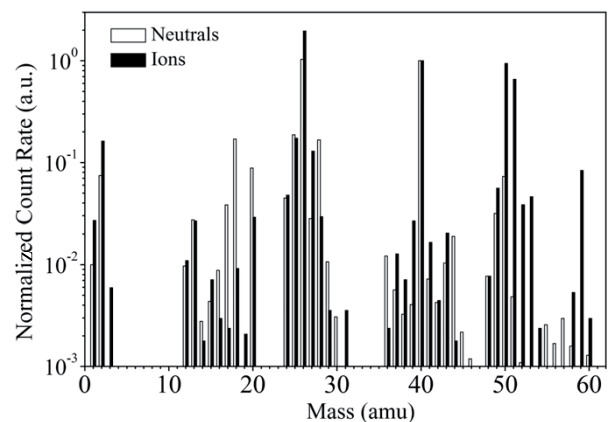
Neutral and ion mass spectra normalised with respect to argon in a CCP at 6 mTorr with 2:1 C_2H_2:Ar ratio.
