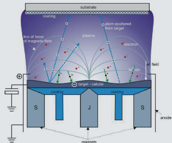
Typical magnetron sputtering arrangement.
