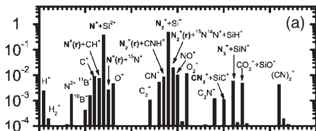
Positive ion spectrum of a silicoboron-carbonitride plasma.
