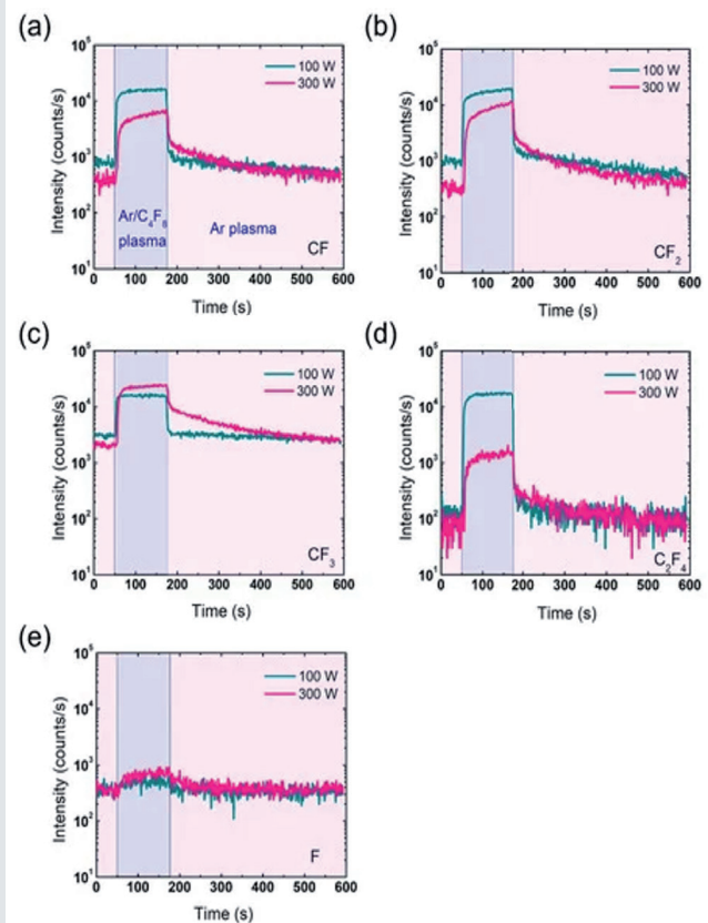
FC radical densities measured using a QMS during one cycle of ALE at 100 W and 300 W of (a) CF, (b) CF 2 , (c) CF 3 , (d) C 2 F 4 , and (e) F.
