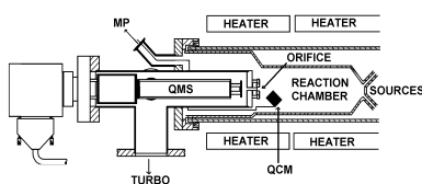
Figure 1. A schematic side view of the reactor.
