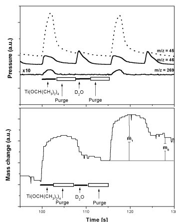
Figure 3. QMS data and QCM mass change in two complete ALD cycles at 250 °C m/z=46 : \text{CH}_3\text{CHOD}^+ , m/z=45 : \text{CH}_3\text{CHOH}^+ , m/z=269 : \text{Ti}(\text{OCH}(\text{CH}_3)_2)_3\text{OCHCH}_3^+
