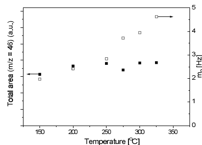
Figure 4. The growth rate measured with QCM ( m_0 ) and the total amount of deuterated reaction products ( m/z = 46 ) measured with QMS.
