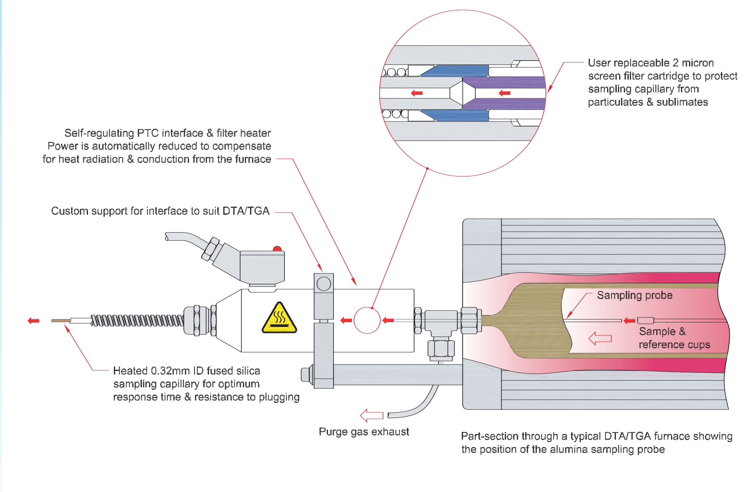
Fig 2. Hidden gas sampling arrangement
